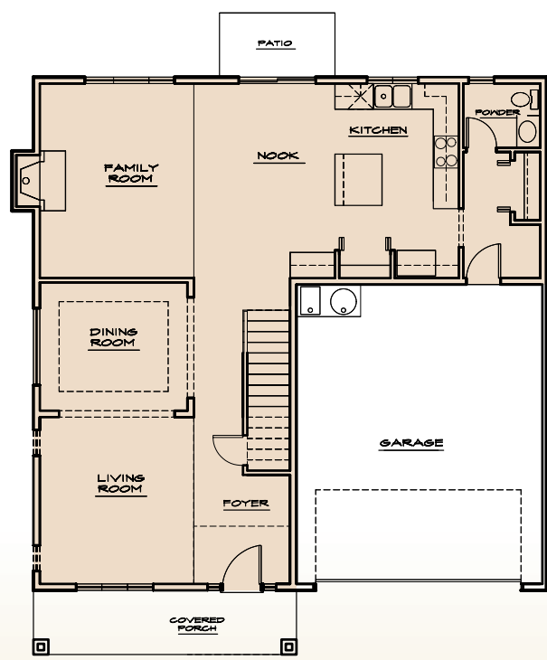
MAIN FLOOR
