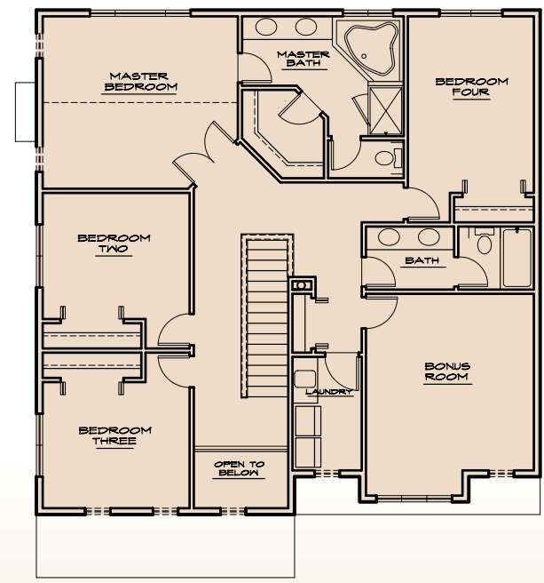
UPPER FLOOR
