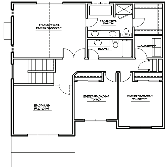
UPPER FLOOR
