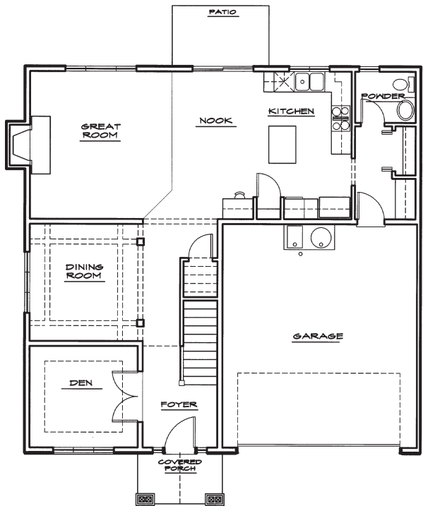
MAIN FLOOR
