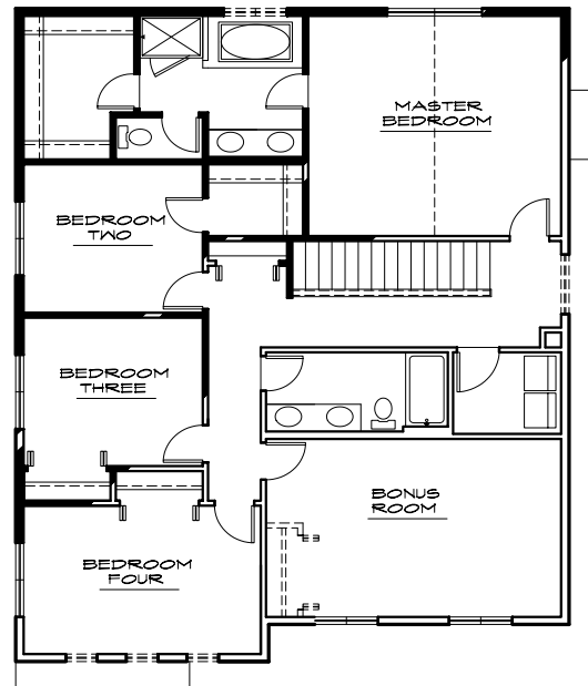
UPPER FLOOR
